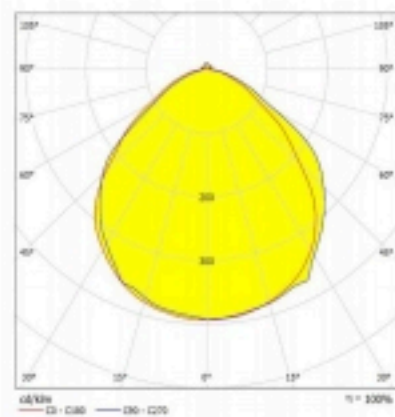
Luminance Distribution
